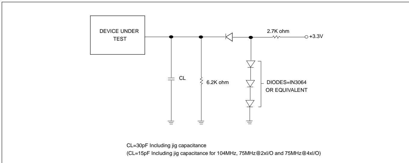
Figure 5. OUTPUT LOADING
